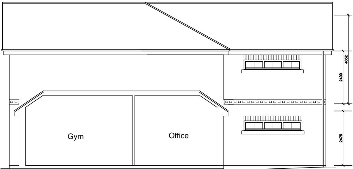
PROPOSED SECTION 1-100
